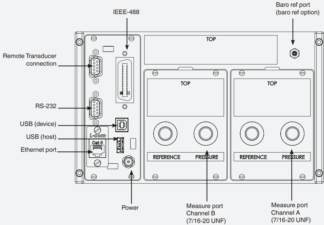
Rear Panel
