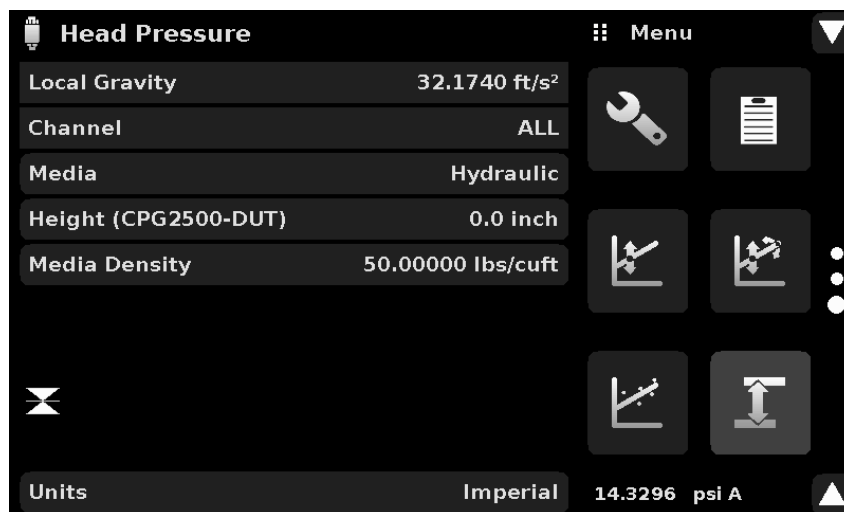
Figure 10.10-D - Head Pressure, Hydraulic
